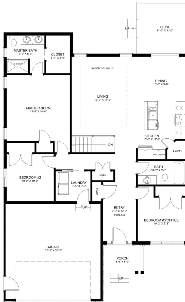
MAIN FLOOR PLAN LIVING AREA = 1458 SQ. FT.
